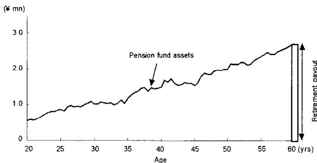
III-1. Change in pension fund assets for one employee under Sundaresan model's simplified plan
