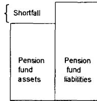
II-3 Pension liabilities exceed assets
