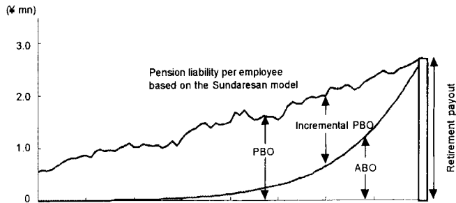
III-2. Change in pension liability for one employee with liability amount calculated as a random variable
