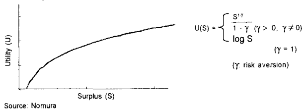
III-3. Utility function
