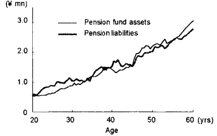
IV-3. Change in pension fund assets (rho = 0)
