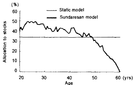
IV-1. Change in allocation to stocks ( \rho = 0 )
