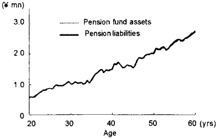
IV-2. Change in pension fund assets (rho = 1)
