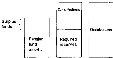
II-2 Relationship of pension fund assets/liabilities and surplus funds
